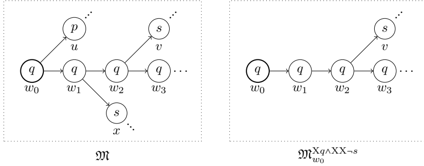
Fig. 2. This figure illustrates how a model is updated and reduced by a formula. The model on the right is the result of updating the one on the left at w_0 with Xq \wedge XX-s .
